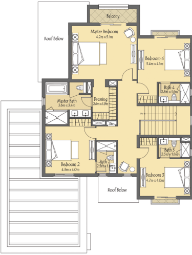
FIRST LEVEL
