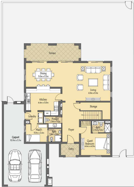
GROUND LEVEL
