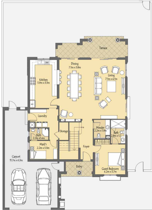
GROUND LEVEL
